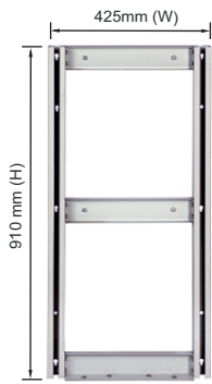
Wall Mounting Stand 425mm (W) x 910mm (H)
