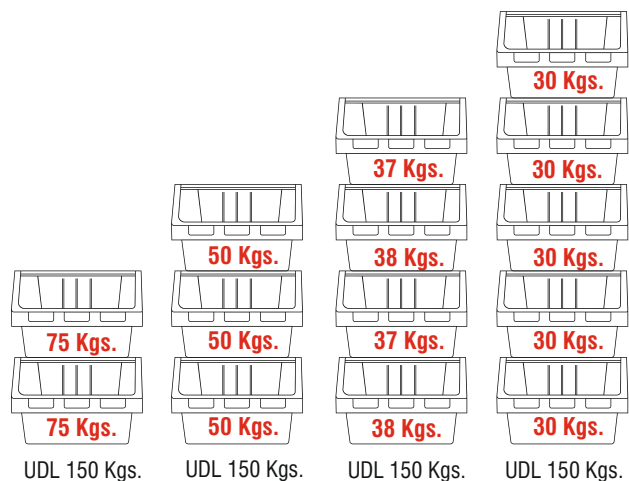
Uniform distributed load bearing capacity of SB-8 at different stack heights
